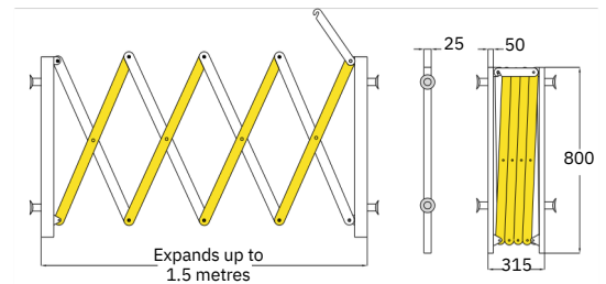
Opens automatically via internal spring mechanism
