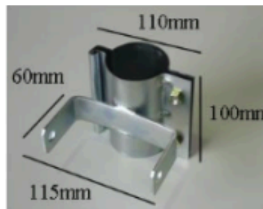
POST MOUNT BRACKET (MIRROR B- POST)
